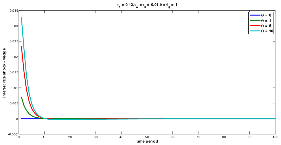
Figure 6: The effect of a single period interest rate shock on \Gamma_t
