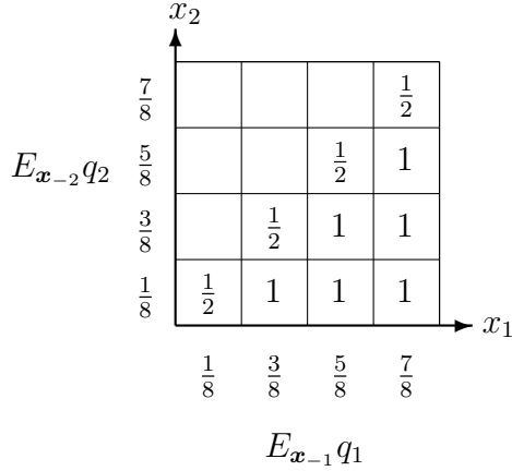
FIGURE 3. An extreme point and its dominant-strategy mechanism
