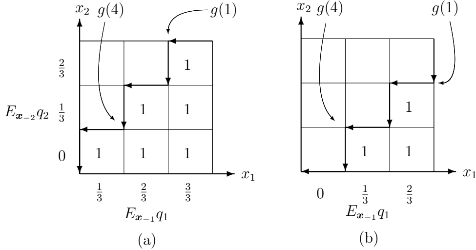
FIGURE 4. Labelings (a) and (b), two extreme points
