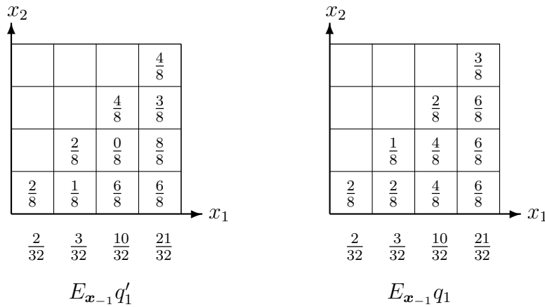
FIGURE 2. In cells with no values, q' and q are 0
