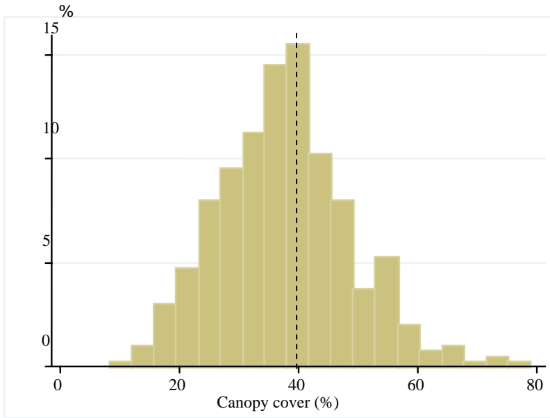
Figure 1: Percentage distribution of forests based on their canopy cover (Indian Himalayas, 2002-3)
