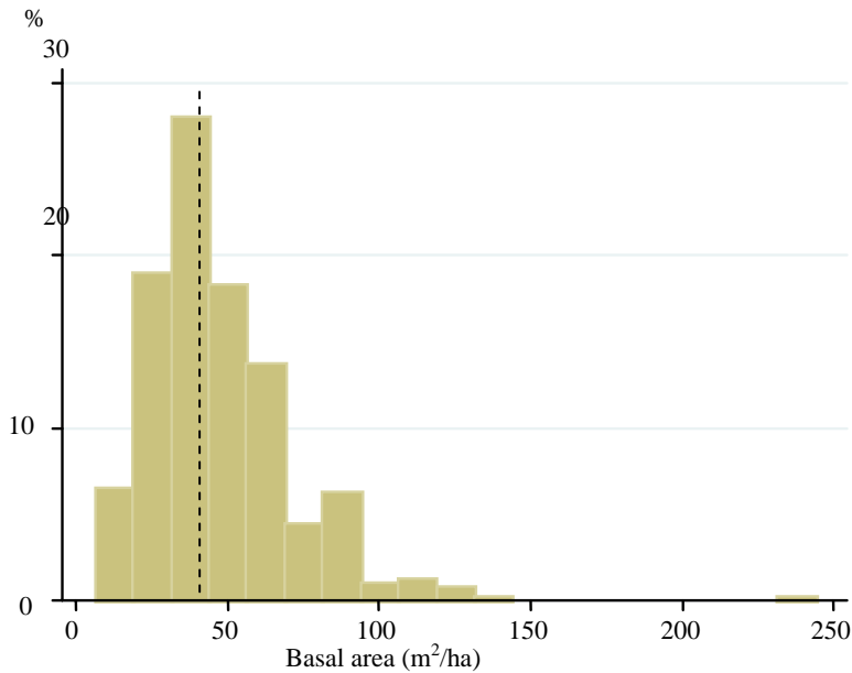
Figure 3: Percentage distribution of forests based on basal area (m 2 /ha) (Indian Himalayas, 2002-3)
