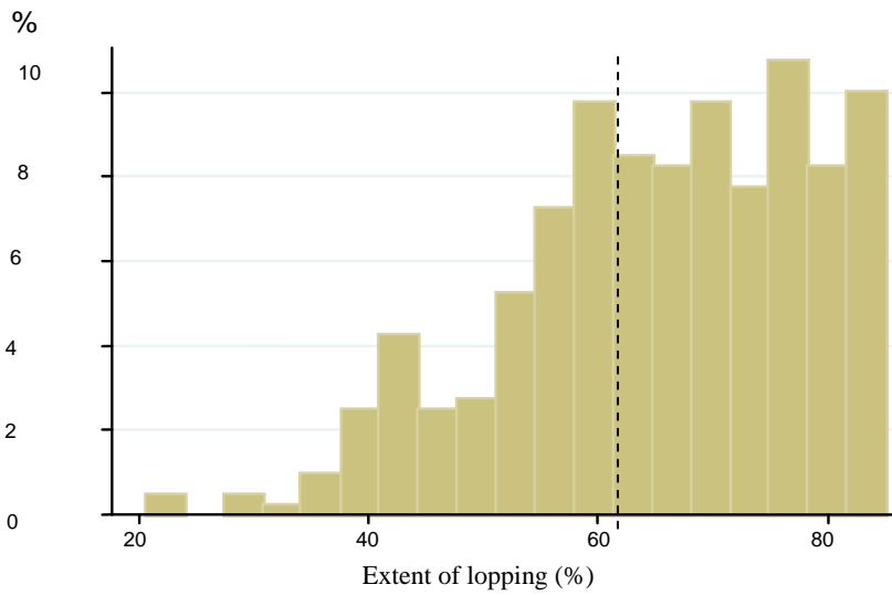
Figure 2: Percentage distribution of forests based on the extent of lopping (Indian Himalayas, 2002-3)
