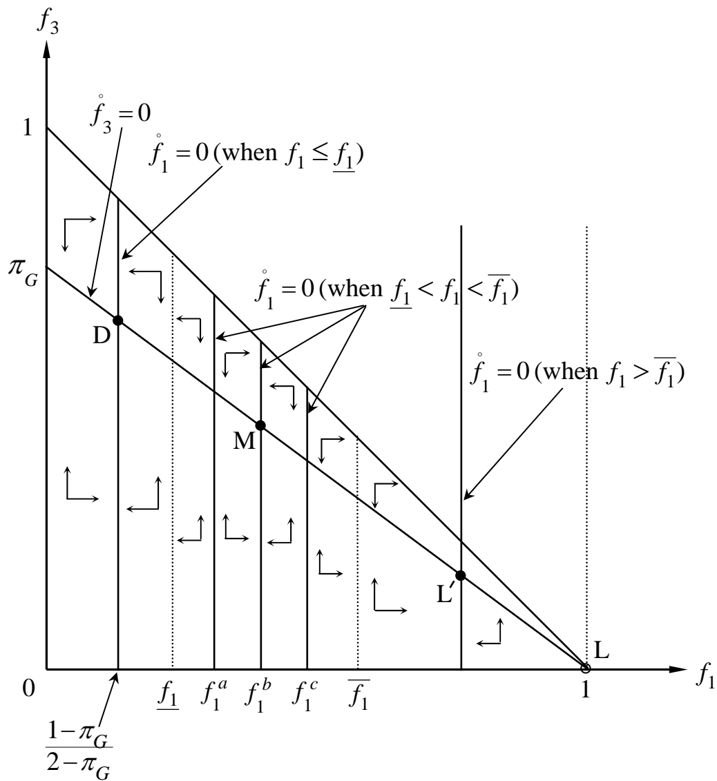
Figure 3(c): Phase Diagram with Perturbed Wealth Dynamics
