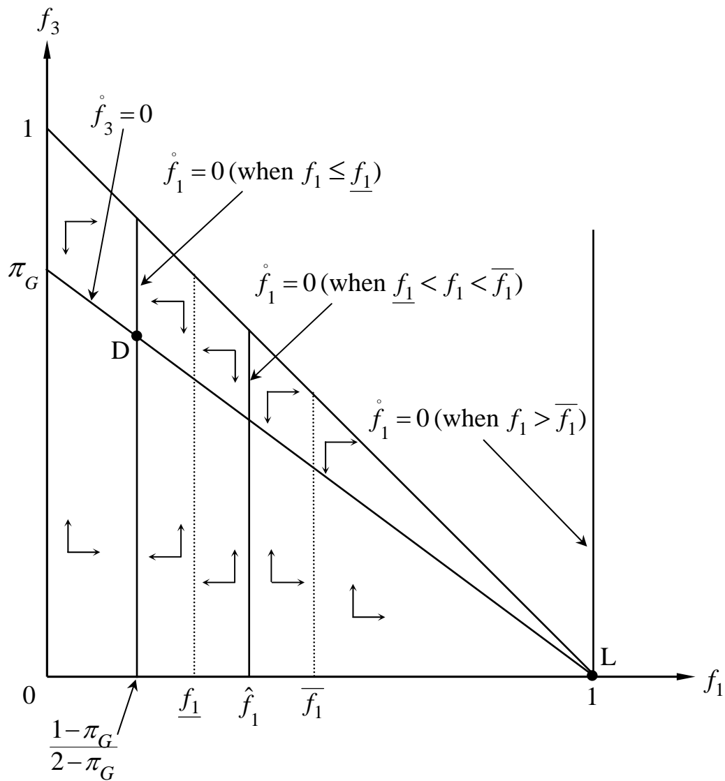
Figure 3(a): Phase Diagram for a single Threshold
