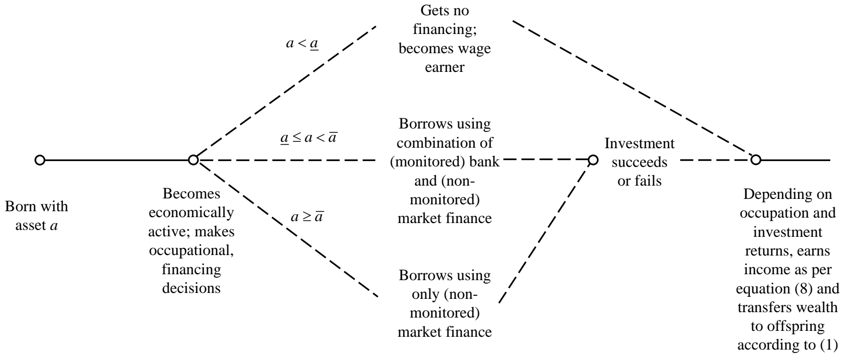
Figure 1: Timeline of Decisions for a Typical Agent
