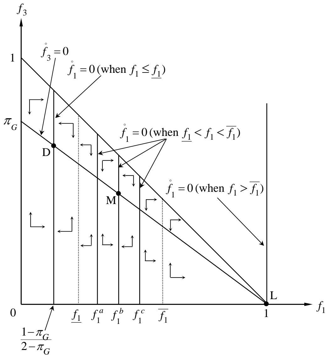
Figure 3(b): Phase Diagram for two Thresholds
