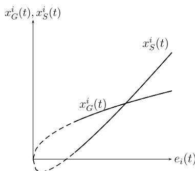
FIGURE 5.—Engel curves. \varepsilon > 0 is assumed. As indicated by the dashed sections, preferences are only well defined if condition (3) holds (i.e., e_i(t) exceeds a certain threshold).
