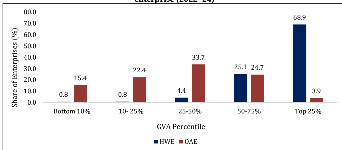
Figure 4.9: Distribution of enterprises across GVA (real) percentiles by type of enterprise (2022–24)
