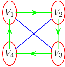
Figure 1: The structure of a singular 3-colored digraph.
