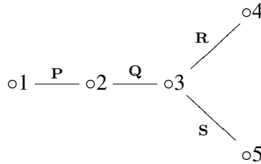
Figure 1: A matrix-weighted tree T .
